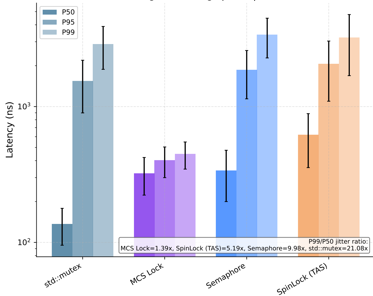
Fig 11 — Tail Latency Comparison: P50 / P95 / P99 (lower is better; large P99 → high jitter) | 95% CI across trials
